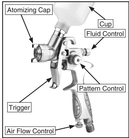
Figure 4. Controls.
